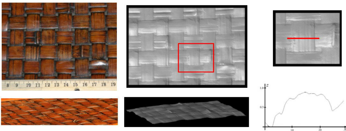
Figure 15: Top left: wooden tabletop with ruler for scale (in centimeters). Top center: plastic shaded reconstruction. Bottom left: oblique view photograph. Bottom center: oblique view reconstruction. Top right: closeup of inset. Bottom right: depth profile of red line in inset, with z-axis scaled up for clarity (axes units are millimeters).
